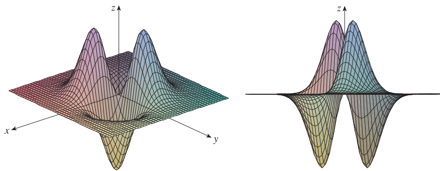
(b) Two views of f(x, y) = -xye^{-x^2 - y^2}
