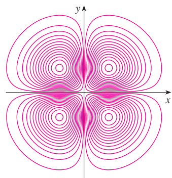
(a) Level curves of f(x, y) = -xye^{-x^2 - y^2}
